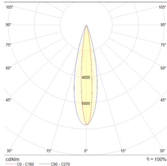
Uplights Lineal 13*25°
