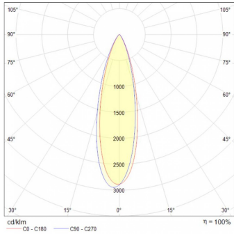
Uplights Lineal 30°
