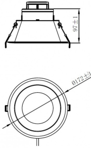
Downlight 28W
