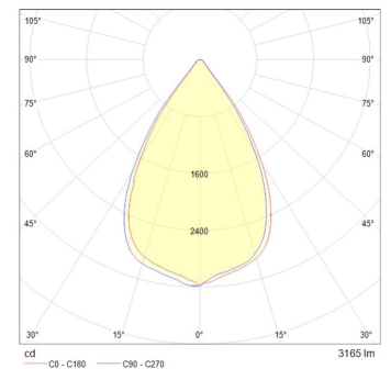
Downlight 34W 60°
