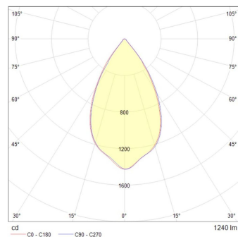
Downlight 14W 60°
