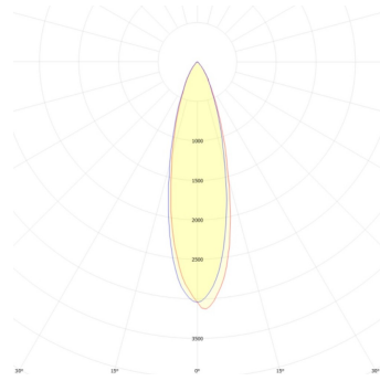
RE1092BBCA 30W
