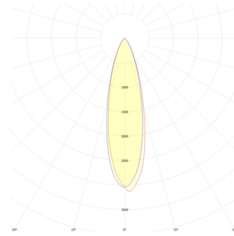
RE1093BBCA 45W
