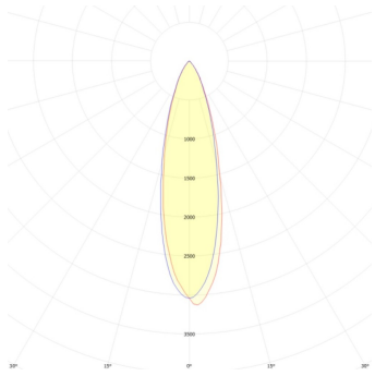
RE1091BBCA 15W
