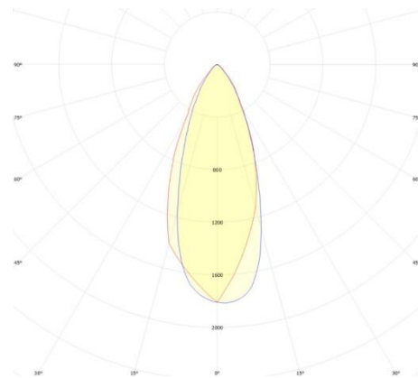
OF4352BBNA/ OF4352NBNA 30 W 4000K 80°
