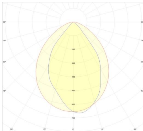
OF4350BCCA/ OF4350NCCA 30 W 4000K 80°
