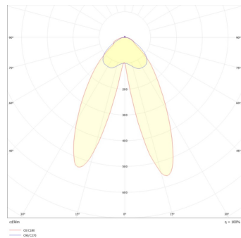
Skylight 20°*120°
