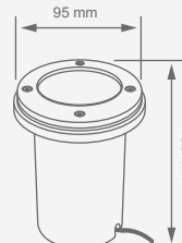
RE8200C00K Base Gx5.3
