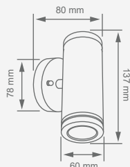
OU7014C00K Base G4
